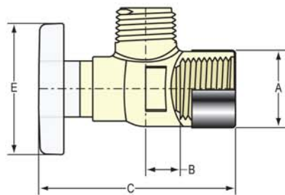
1/4-Turn Angle Supply Stop SR FiPT x NPT/Compression
